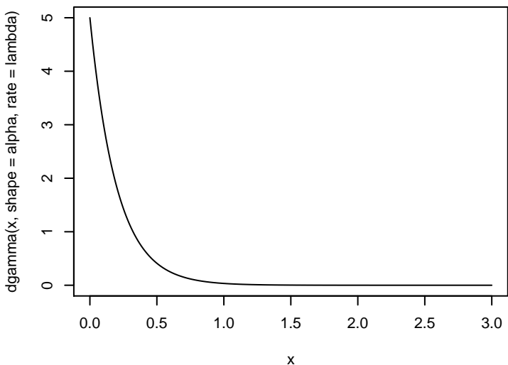
Density of Gamma(1,5)
