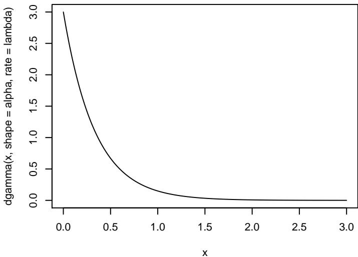
Density of Gamma(1,3)
