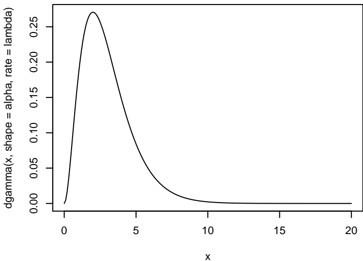
Density of Gamma(3,1)
