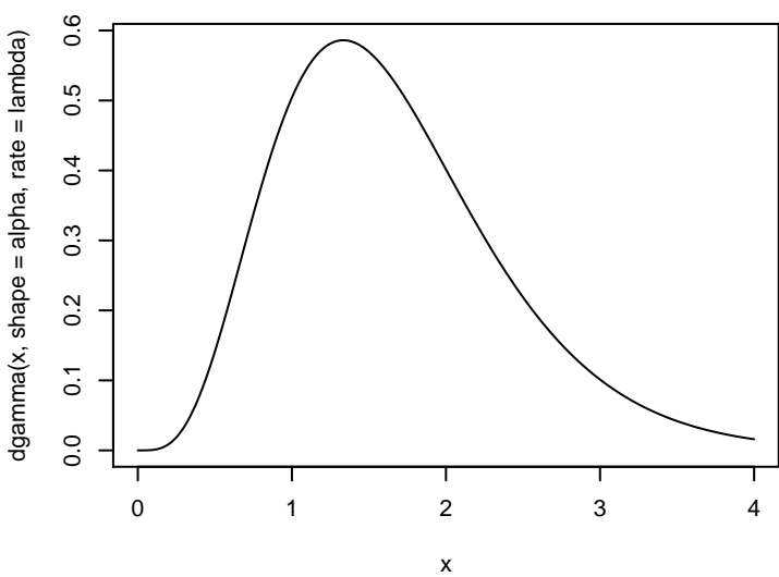
Density of Gamma(5,3)
