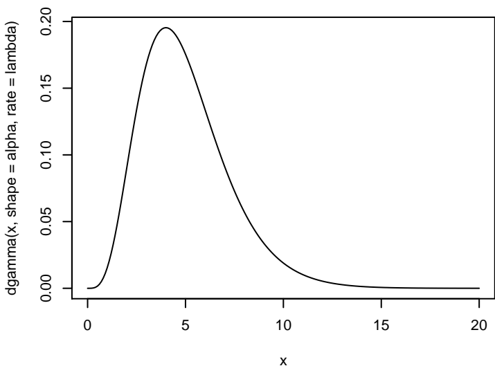
Density of Gamma(5,1)
