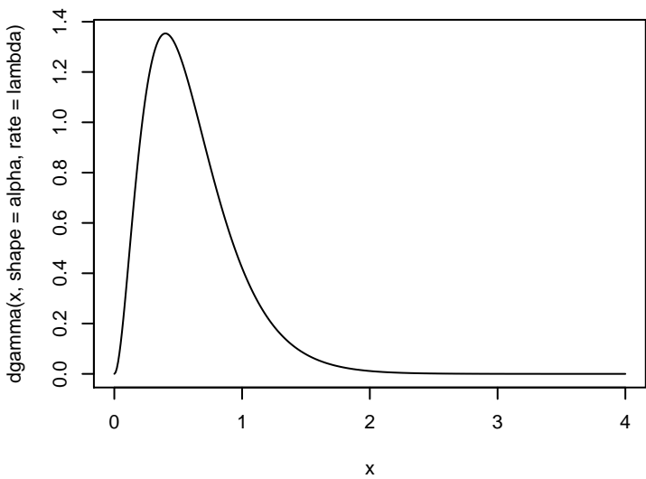
Density of Gamma(3,5)
