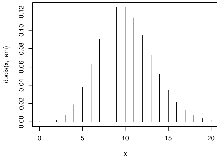
Density of Poisson(10)
