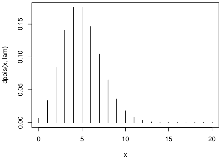
Density of Poisson(5)
