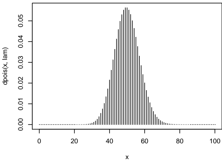
Density of Poisson(50)
