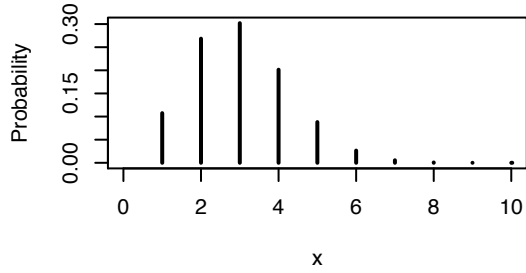
Bin(n=10, p=0.2)
