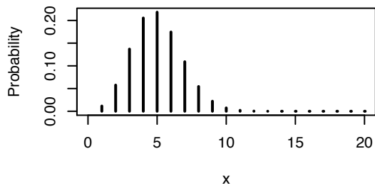
Bin(n=20, p=0.2)
