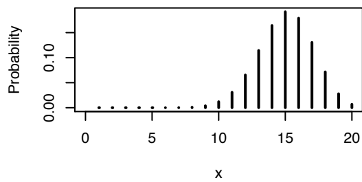
Bin(n=20, p=0.7)
