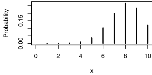
Bin(n=10, p=0.7)
