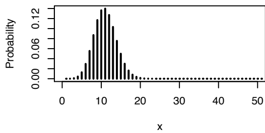
Bin(n=50, p=0.2)
