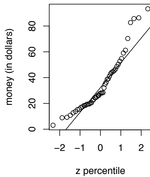
Normal Probability Plot
