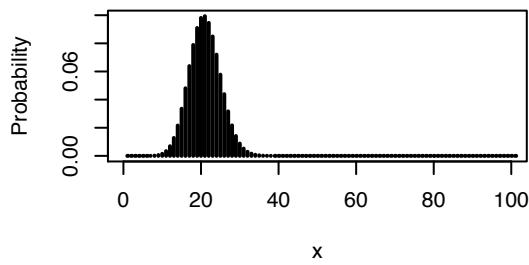
Bin(n=100, p=0.2)
