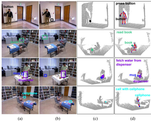
Figure 9. Object recognition and localization. (a) Ground truth. (b) HOG. (c) RDH. (d) Our 4DHOI. The results of RDH are visualized by projecting the areas on the depth images into the 3D point cloud.
