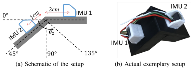
Fig. 7: Experimental setup for evaluating the angle reconstruction with two articulated IMUs
