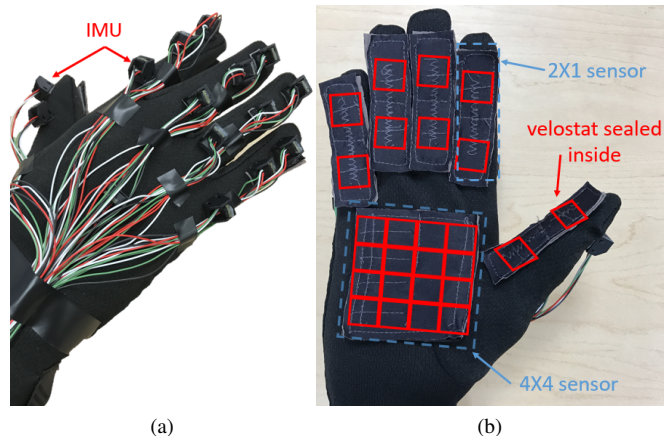
Fig. 1: Prototype consisting of (a) 15 IMUs on the dorsum of the hand and (b) 6 integrated Velostat force sensor with 26 taxels on the palmar aspects of the hand.
