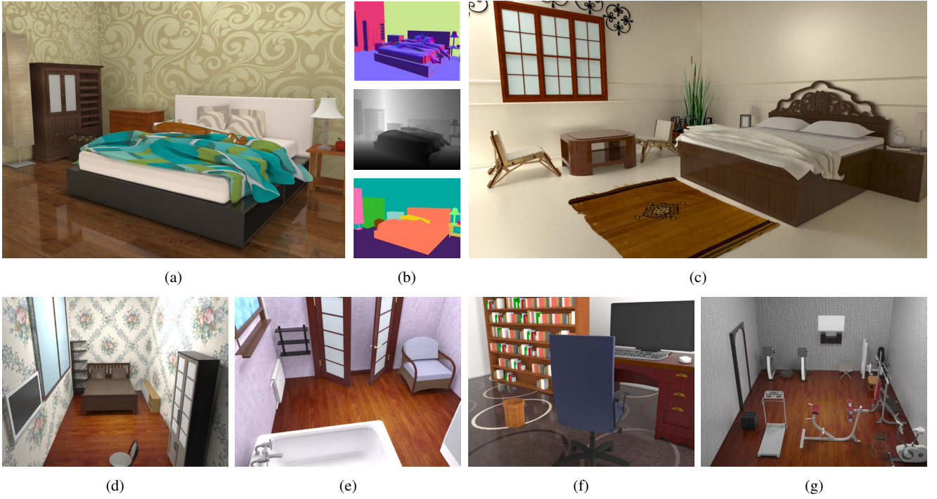
Fig. 1: (a) An example automatically-generated 3D bedroom scene, rendered as a photorealistic RGB image, along with its (b) per-pixel ground truth (from top) surface normal, depth, and object identity images. (c) Another synthesized bedroom scene. Synthesized scenes include fine details—objects ( e.g. , duvet and pillows on beds) and their textures are changeable, by sampling the physical parameters of materials (reflectance, roughness, glossiness, etc. ), and illumination parameters are sampled from continuous spaces of possible positions, intensities, and colors. (d)–(g) Rendered images of four other example synthetic indoor scenes—(d) bedroom, (e) bathroom, (f) study, (g) gym.
