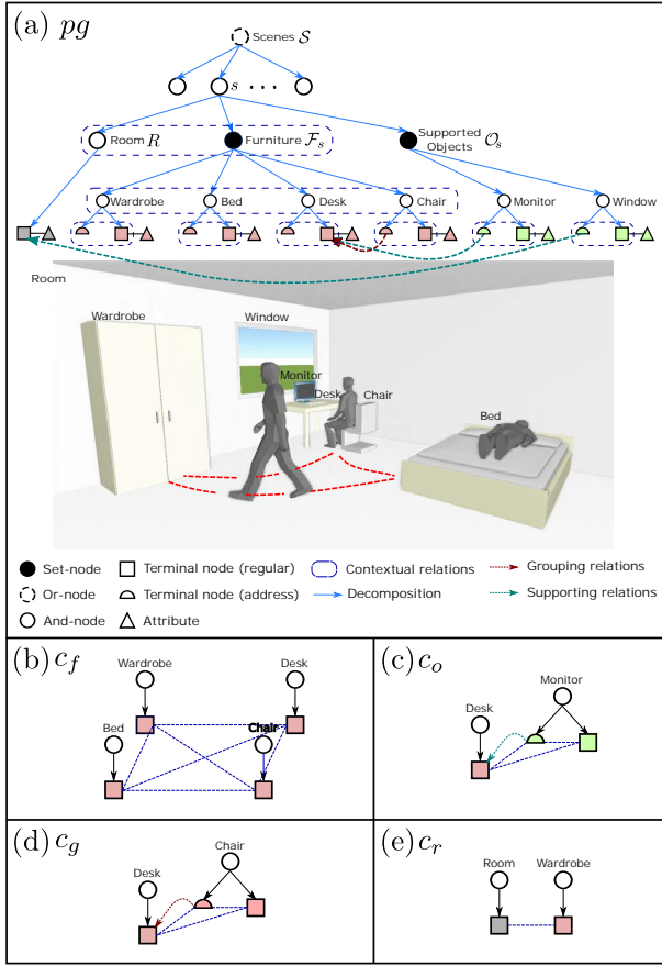
Fig. 3: (a) A simplified example of a parse graph of a bedroom. The terminal nodes of the parse graph form an MRF in the bottom layer. Cliques are formed by the contextual relations projected to the bottom layer. (b)–(e) give an example of the four types of cliques, which represent different contextual relations.
