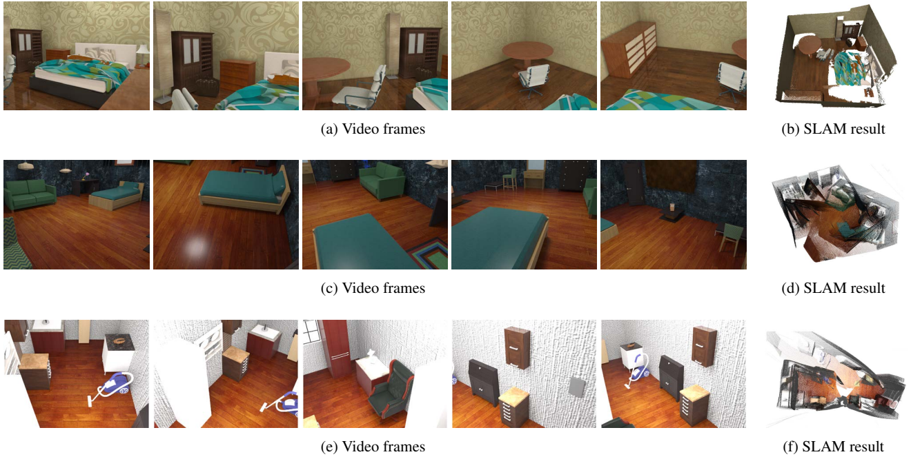
Fig. 10: Specifying camera trajectories, we can render scene fly-throughs as sequences of video frames, which may be used to evaluate SLAM reconstruction [132] results; e.g. , (a) (b) a successful reconstruction case and two failure cases due to (c) (d) a fast moving camera and (e) (f) untextured surfaces.
