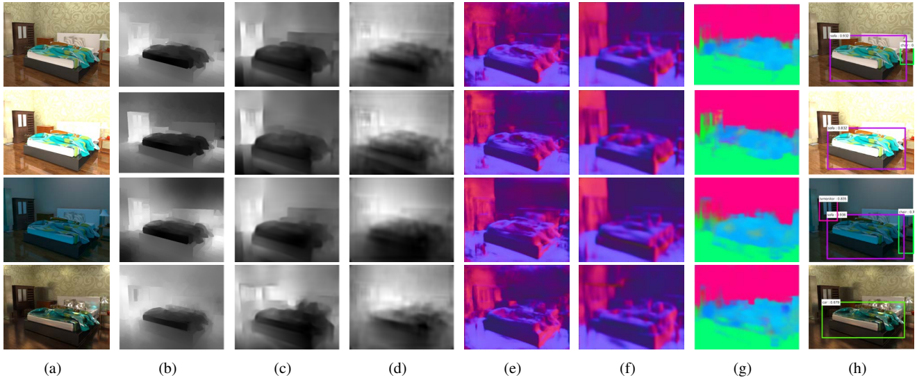
Fig. 11: Benchmark results. (a) Given a set of generated RGB images rendered with different illuminations and object material properties—from top) original settings, high illumination, blue illumination, metallic material properties—we evaluate (b)–(d) three depth prediction algorithms, (e)–(f) two surface normal estimation algorithms, (g) a semantic segmentation algorithm, and (h) an object detection algorithm.
