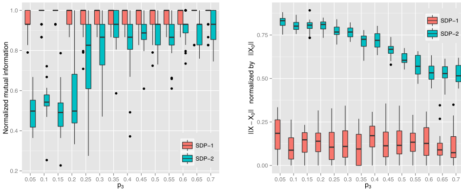
FIG. 4. NMI and relative error of \widehat{X} versus p_3 for the model with probability matrix (8.1).
