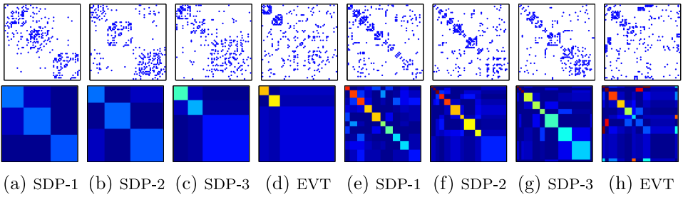
FIG. 5. Results for the dolphins network for K = 3 (a)–(d) and K = 10 (e)–(h). Row 1: adjacency matrix sorted according to the permutation of Algorithm 1. Row 2: Graphon estimator \hat{M}_{\hat{Z}} of Algorithm 1.
