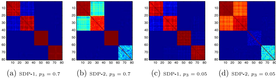
FIG. 3. Mean estimated cluster matrices, \widehat{X} , for SDP-1 and SDP-2, for the weakly but not strongly assortative model (8.1) with p_3 = 0.7 and p_3 = 0.05 . SDP-2 fails to recover one block at p_3 = 0.7 and two blocks at p_3 = 0.05 .
