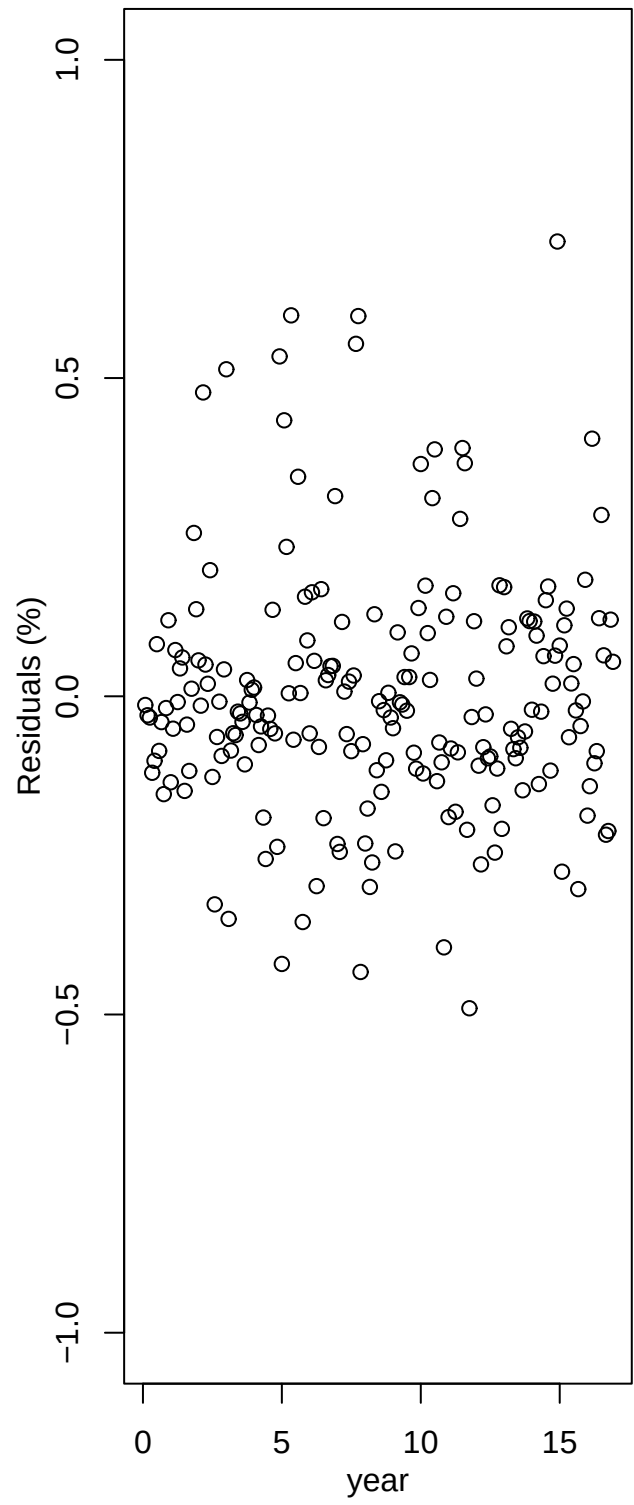
Fig 12: ARIMA (1,0,0) Residuals
