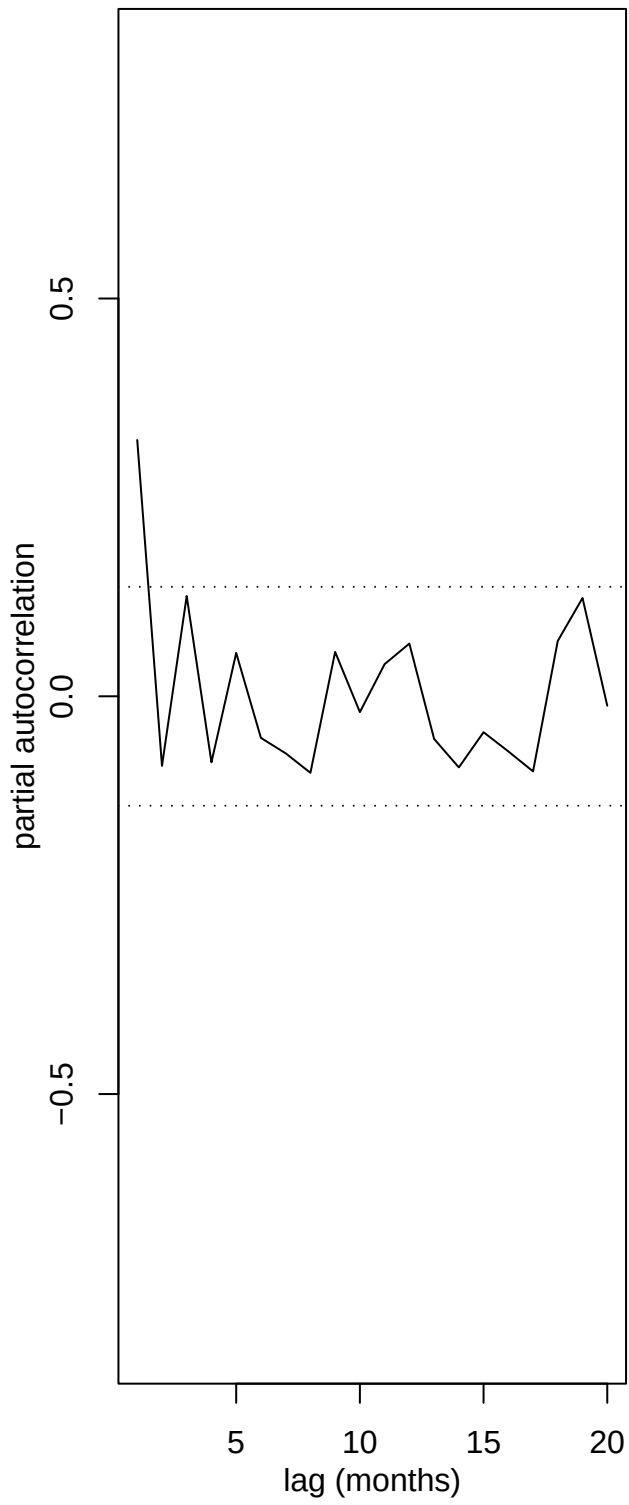
Fig 11: Partial ACF of first differences
