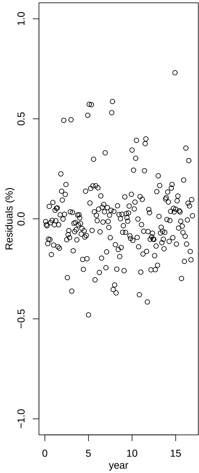
Fig 14: ARIMA (1,0,1) Residuals
