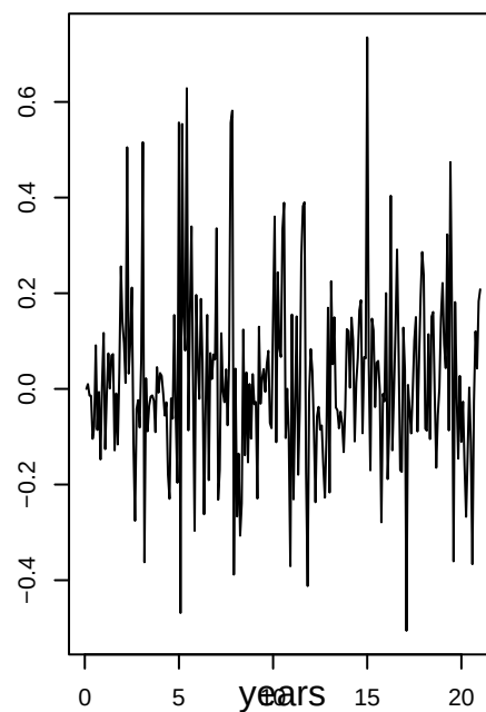
Fig 17: Data, ARIMA(0,1,1) fit, & prediction errors
