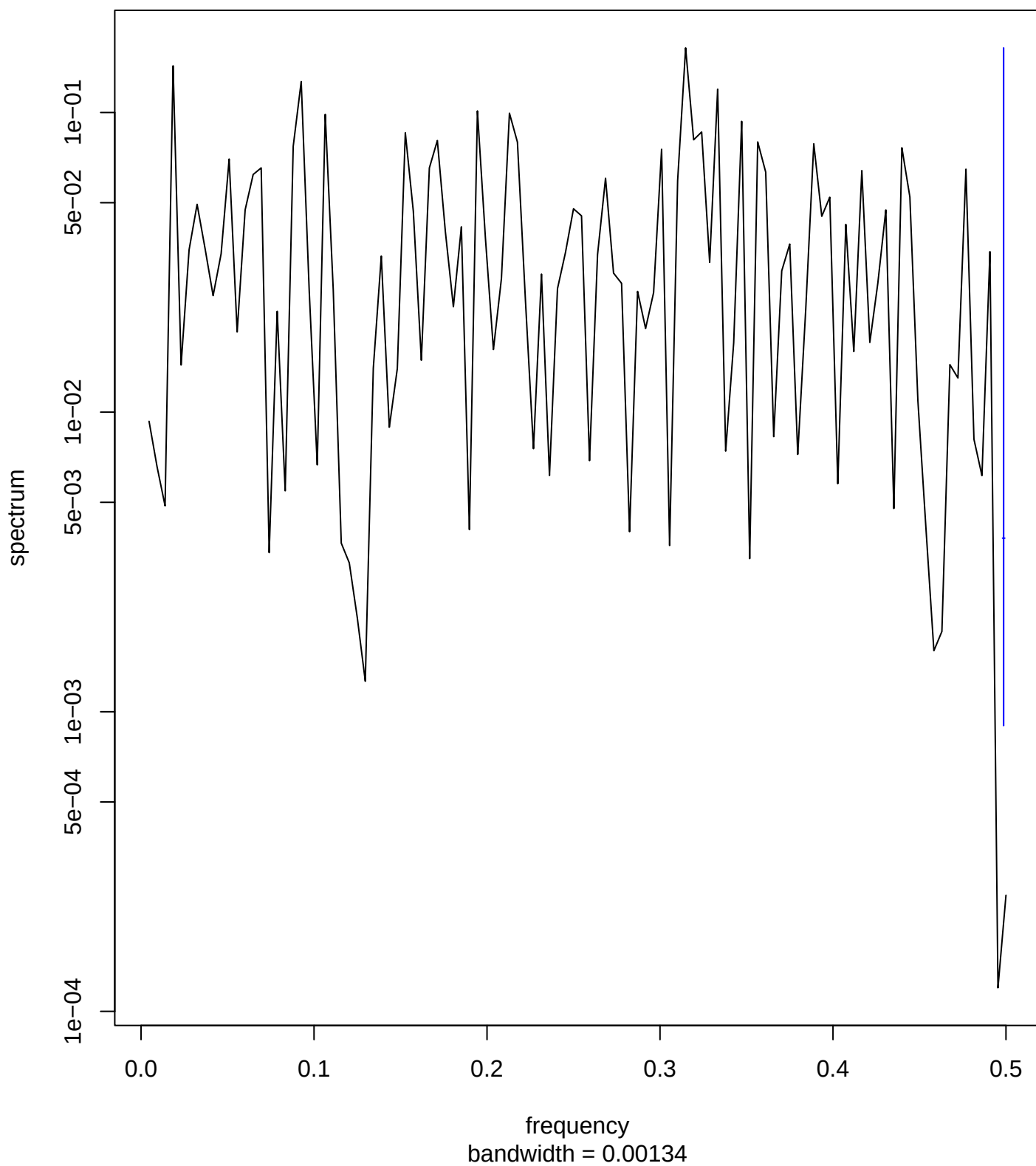
Series: res1 Raw Periodogram
