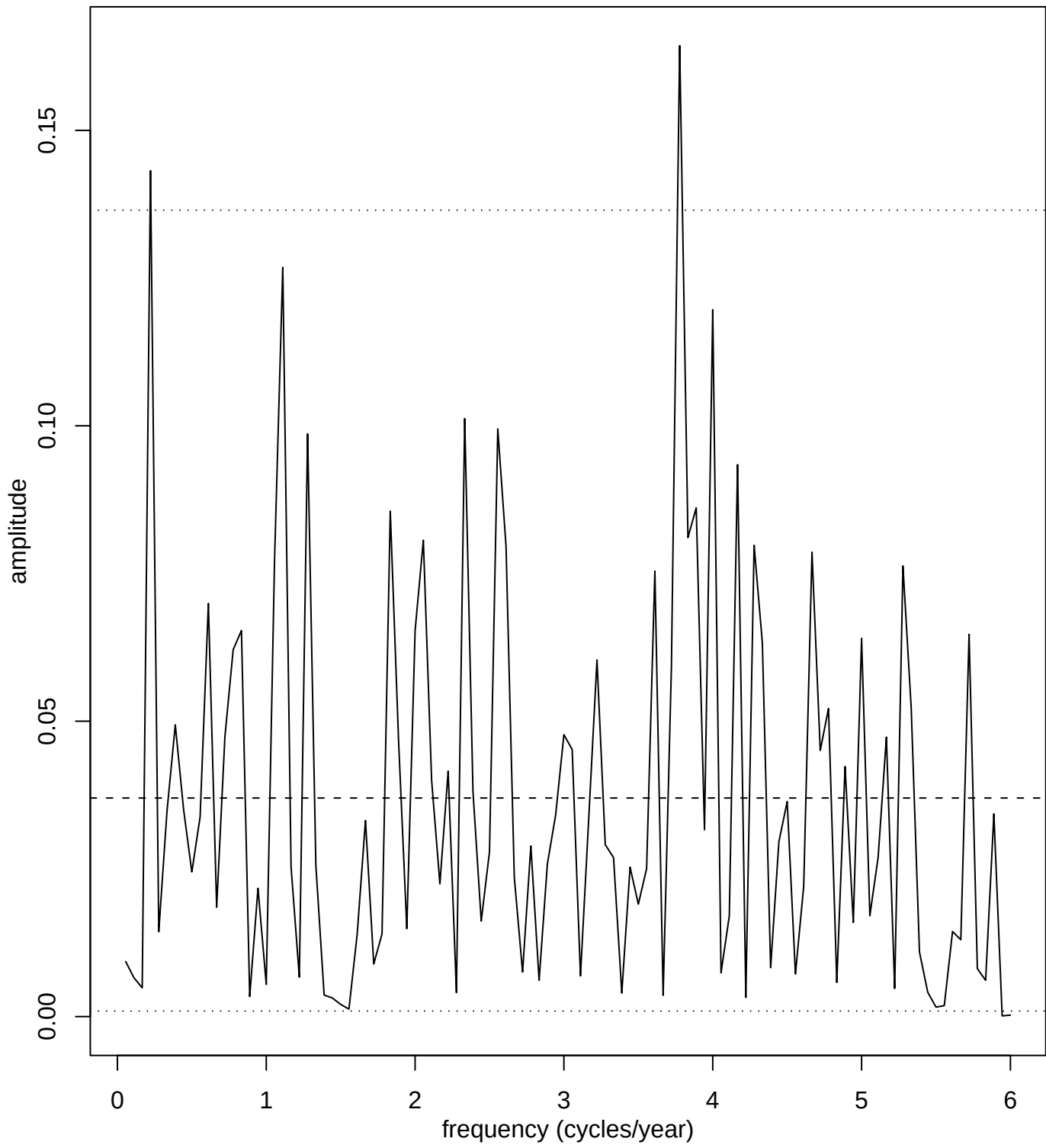
Fig 21: Periodogram of ARIMA(0,1,1) resid
