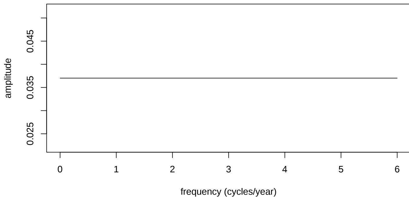
Fig 23: AR-spectrum estimate of ARIMA(0,1,1) resids
