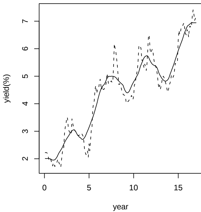
Fig 9: time-plot with simple MA(2*12+1) filter
