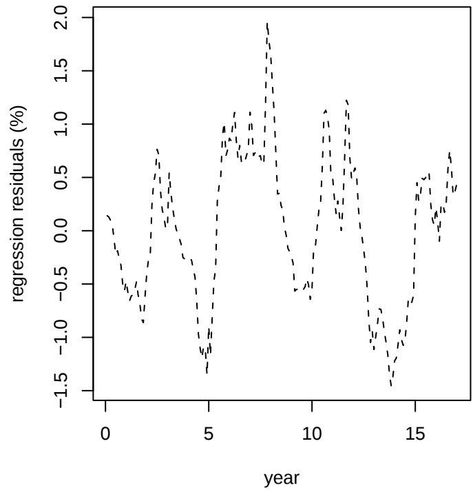
Fig 8: Linear regression residuals
