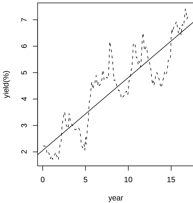
Fig 7: Time plot with regression line
