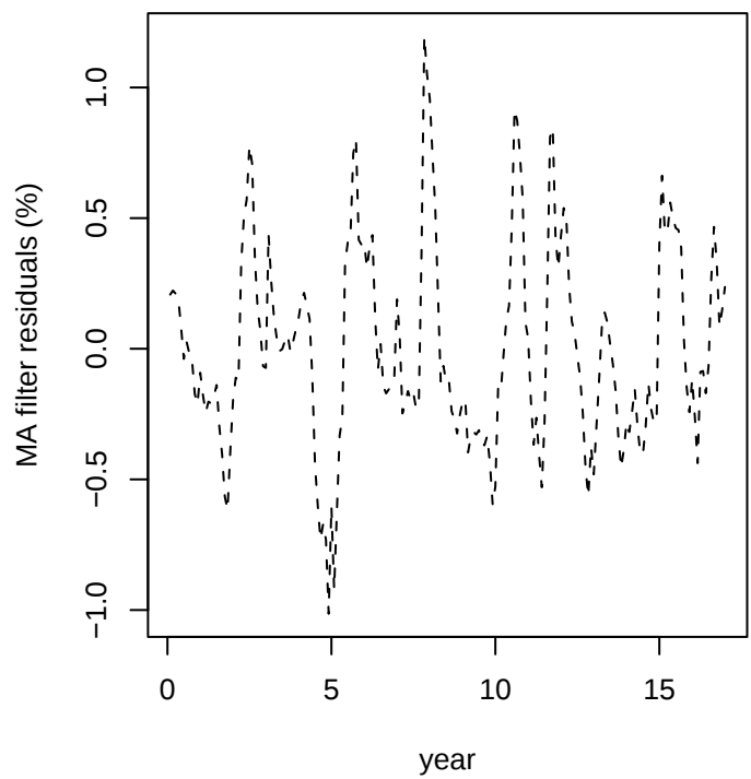
Fig 10: MA(2*12+1) filter residuals
