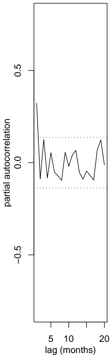
Fig 11: Partial ACF of first differences
