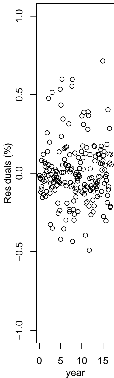
Fig 12: ARIMA (1,0,0) Residuals
