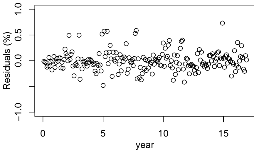
Fig 14: ARIMA (1,0,1) Residuals
