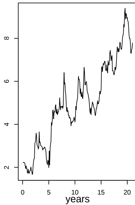
ARIMA(0,1,1) fit
