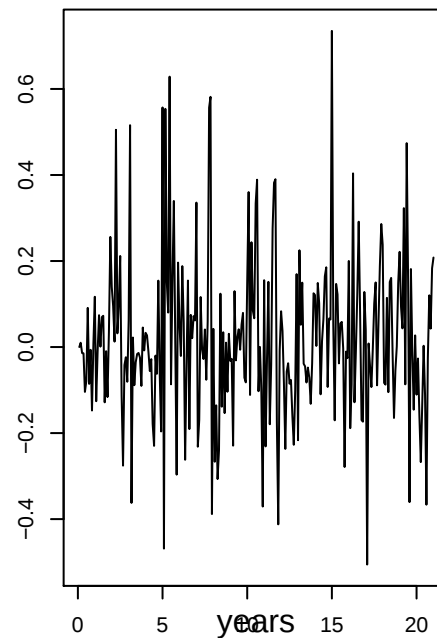
prediction errors
