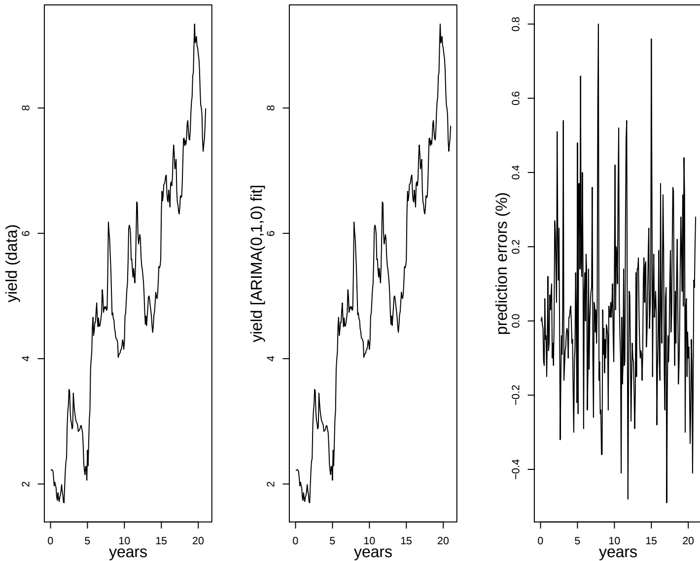
Fig 18: Data, ARIMA(0,1,0) fit, & prediction errors
