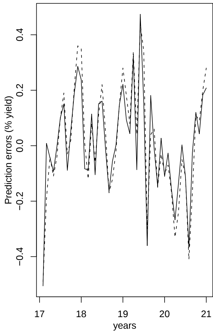
Fig 19: Prediction errors solid = ARIMA(0,1,1). dotted = ARIMA(0,1,0).
