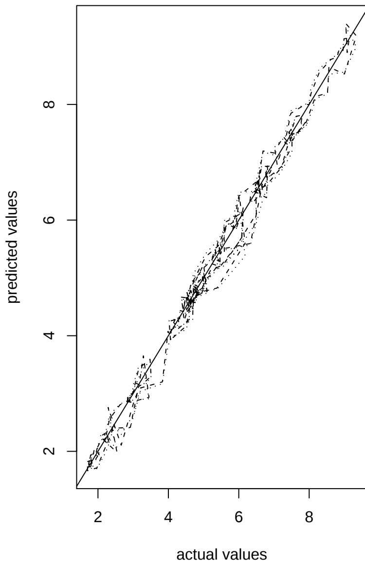
Fig 20. dashed = ARIMA(0,1,1). dotted = ARIMA(0,1,0).
