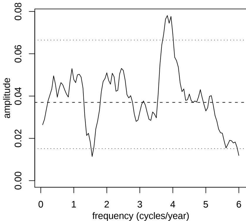
Fig 22: Smoothed p-gram of ARIMA(1,1,0) resid
