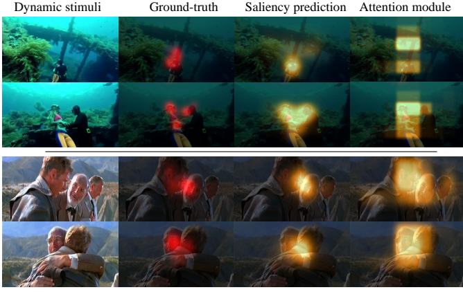
Fig. 5. Illustration of the attention maps predicted from our ACLNet and the attention module on two dynamic stimuli. Best viewed in color.
