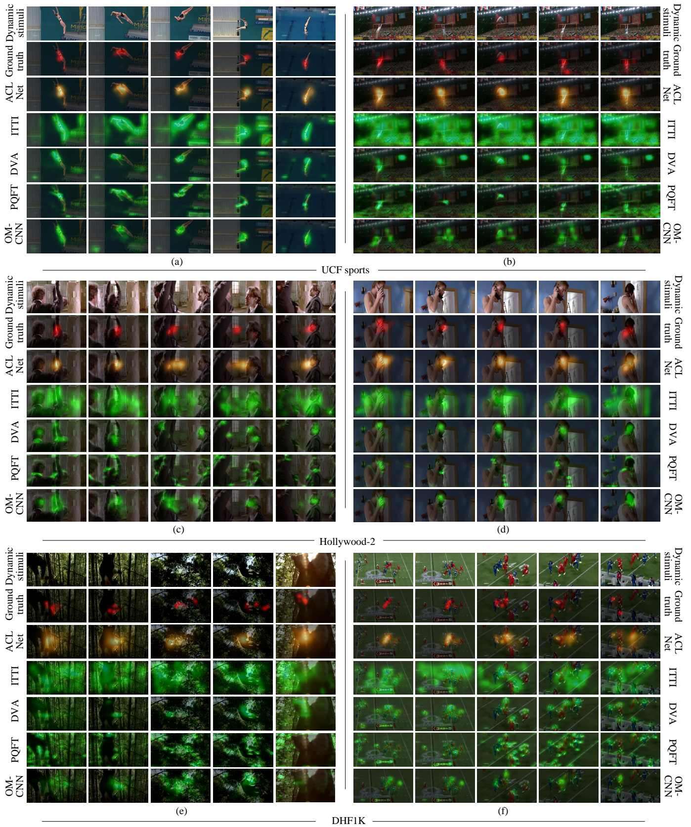
Fig. 7. Qualitative results of our ACLNet and four representative saliency models: ITTI [26] (non-deep static saliency model), DVA [29] (deep static saliency model), PQFT [10] (non-deep dynamic saliency model), and OM-CNN [24] (deep dynamic saliency model) on three video saliency datasets: UCF sports [35] (a, b), Hollywood-2 [35] (c, d) and DHF1K (e, f). Best viewed in color. It can be observed that the proposed ACLNet is able to handle various challenging scenes well and produces more accurate video saliency results than other competitors. See Sec. 5.5 for details.
