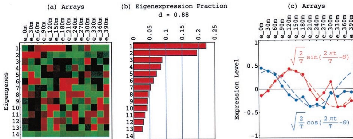
Fig. 1. Normalized elutriation eigengenes. (a) Raster display of \hat{v}_{LV}^T , the expression of 14 eigengenes in 14 arrays. (b) Bar chart of the fractions of eigenexpression, showing that |\gamma_1\rangle_N and |\gamma_2\rangle_N capture about 20% of the overall normalized expression each, and a high entropy d = 0.88 . (c) Line-joined graphs of the expression levels of |\gamma_1\rangle_N (red) and |\gamma_2\rangle_N (blue) in the 14 arrays fit dashed graphs of normalized sine (red) and cosine (blue) of period T = 390 min and phase \theta = 2\pi/13 , respectively.
