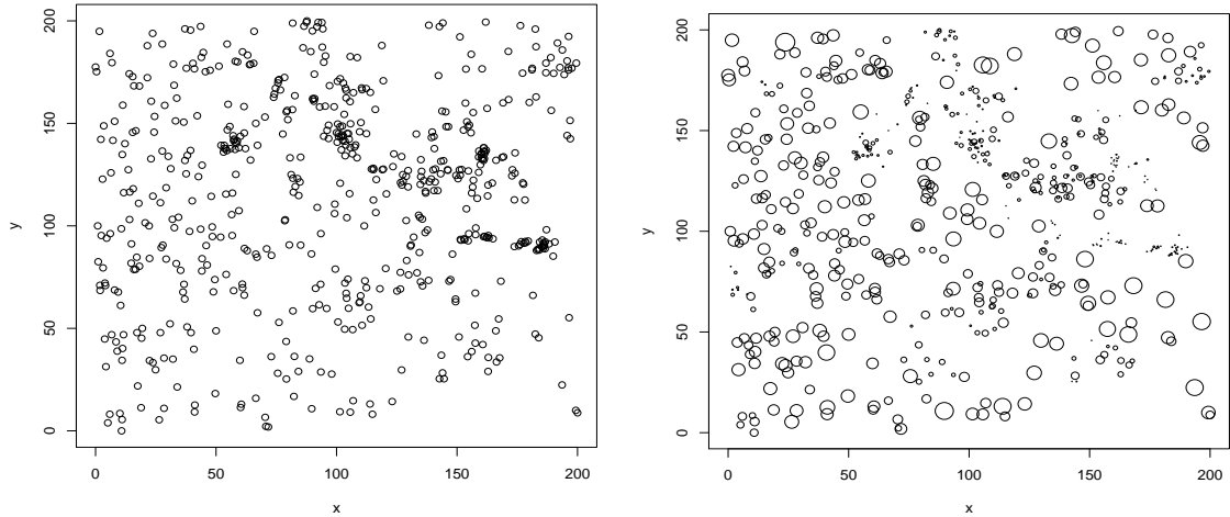
Unmarked and marked point pattern data.
