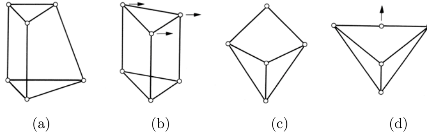
Figure 11.3. Rigid and nonrigid structures.
