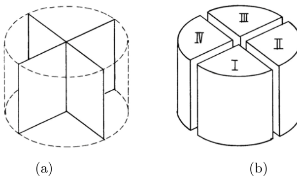
Figure 2.5. Four quadrants generated by two mutually intersecting planes: (a) shows two planes intersecting at a line, and (b) shows the four quadrants generated by the two planes.
