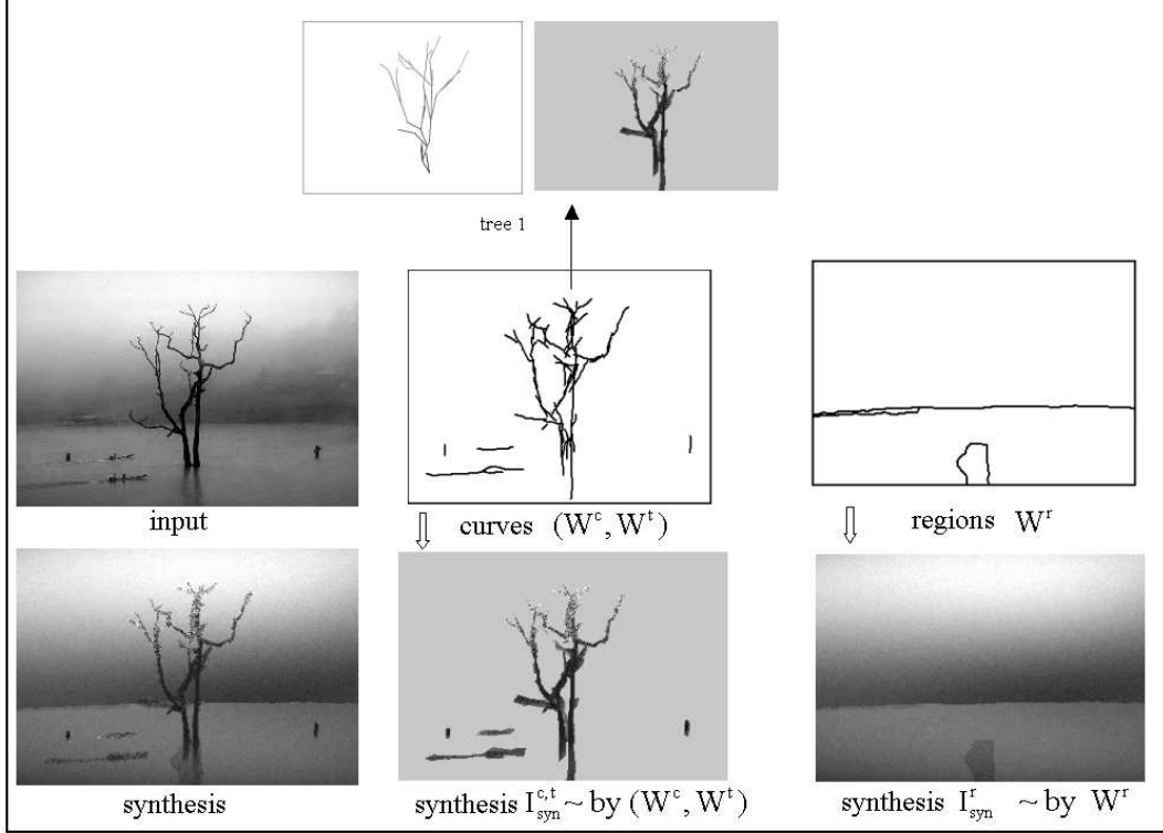
Figure 22: Experiment B3: parsing a tree image into regions, curves, and trees
