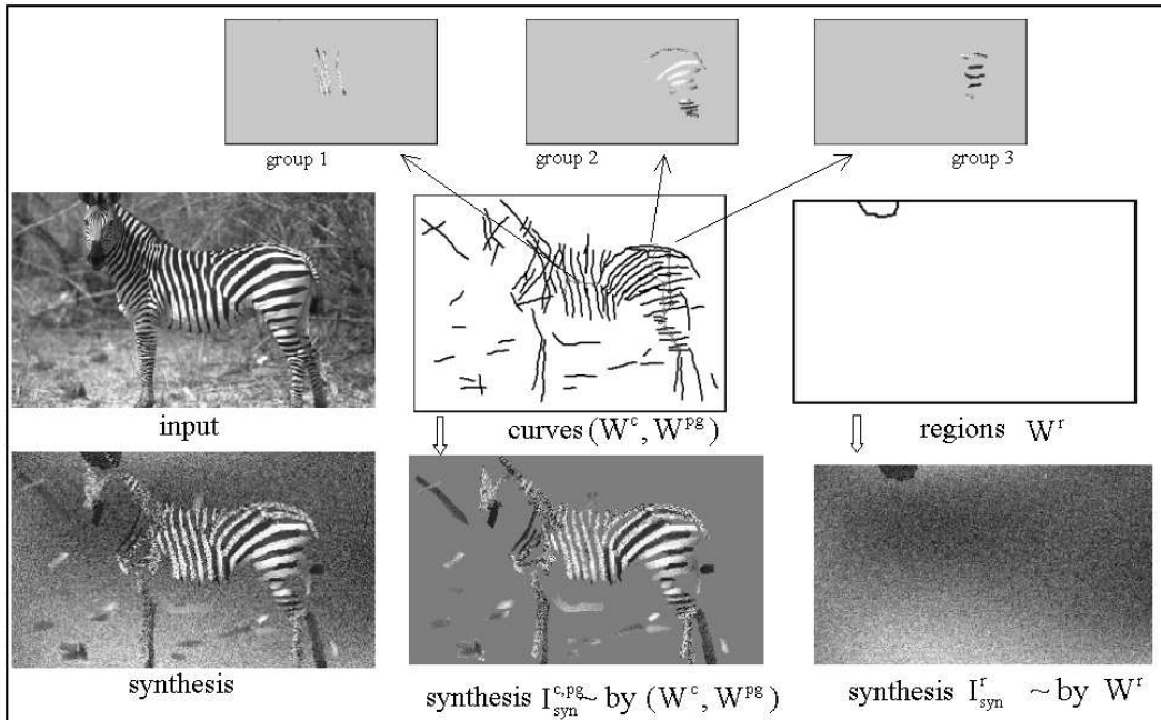
Figure 21: Experiment B2: parsing an image into regions, curves, and parallel curve groups.
