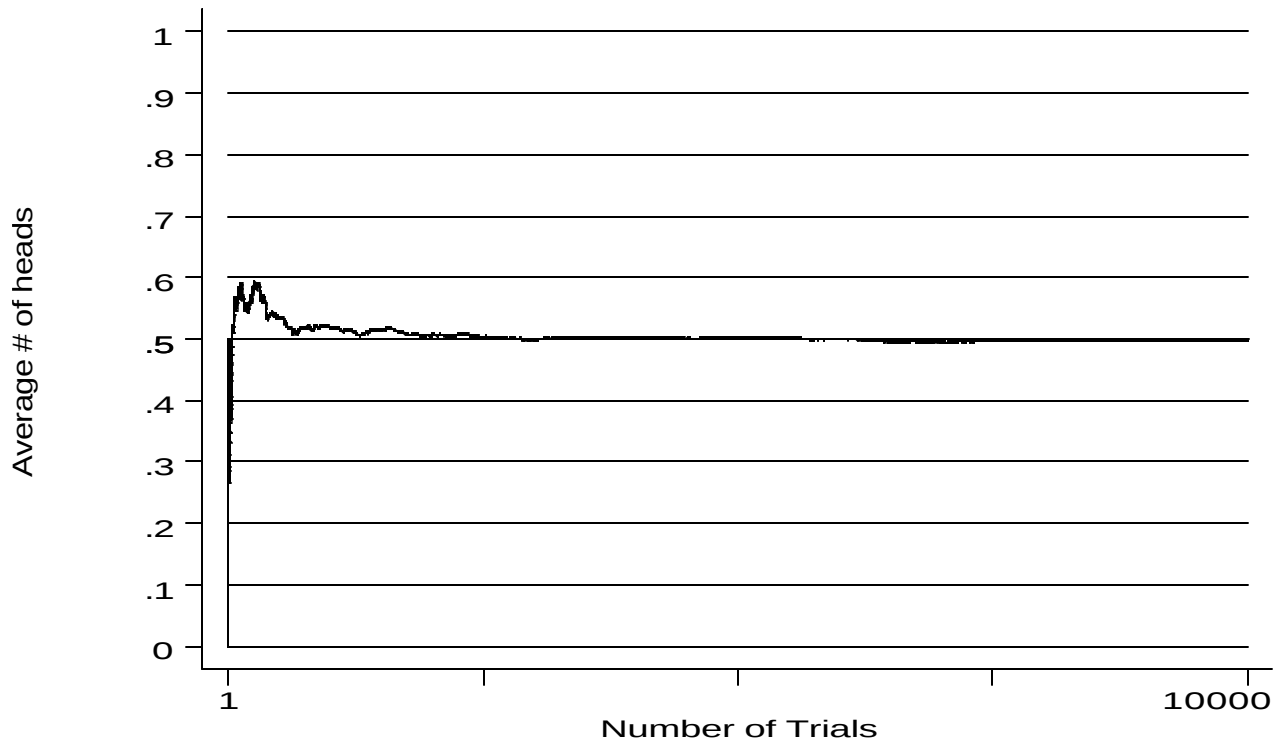
Graph of average number of heads from trial 1 to 10000 of 1 coins with p(\text{head})=.5
