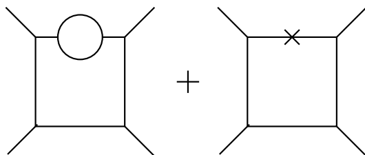
Figure 18.1: The one-loop contribution to V_4 .
