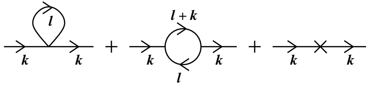
Figure 31.4: O(\lambda) corrections to the \rho propagator.
