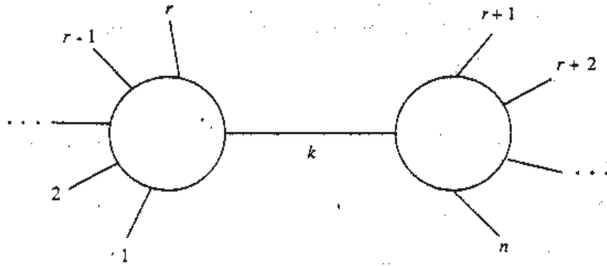
Figure 10.2. A Feynman diagram with the pole structure (10.2.6). Here the line carrying a momentum k represents an elementary particle, one whose field appears in the Lagrangian.
