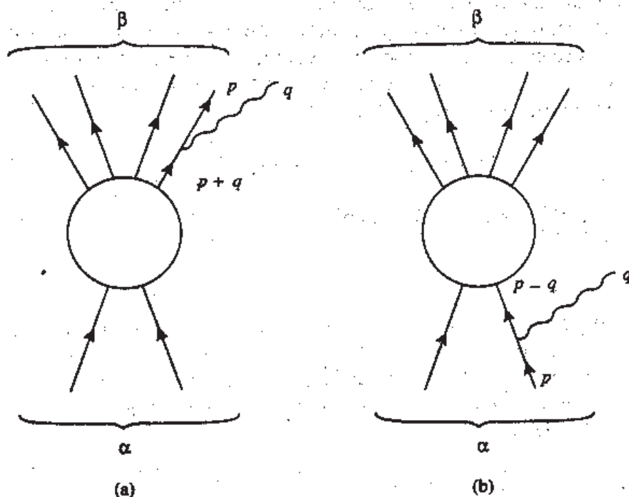
Figure 13.1. Dominant graphs for the emission of soft photons in an arbitrary process \alpha \rightarrow \beta . Straight lines are particles in the states \alpha and \beta (including possible hard photons); wavy lines are soft photons.
