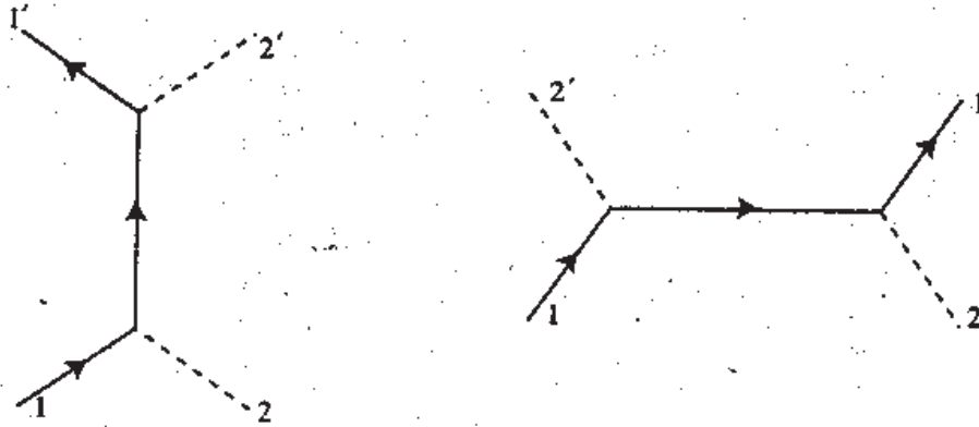
Figure 6.6. The connected second-order diagrams for boson-fermion scattering in a theory with interaction (6.1.18). Straight lines are fermions; dashed lines are neutral bosons.
