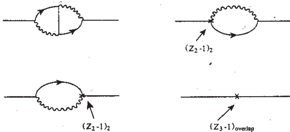
Figure 12.3. Some fourth-order graphs for the electron self-energy in quantum electrodynamics that involve overlapping divergences. Wavy lines are photons; other lines are electrons. The crosses mark the contribution of counterterms.
