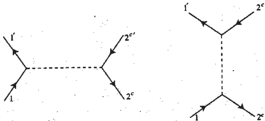
Figure 6.5. The connected second-order diagrams for fermion-antifermion scattering in a theory with interaction (6.1.18). Here straight lines represent fermions or antifermions, depending on the arrow direction; dotted lines are neutral bosons. There is again a minus sign difference in the contributions of these two diagrams, arising from an extra interchange of fermion operators in the pairings represented by the second diagram.
