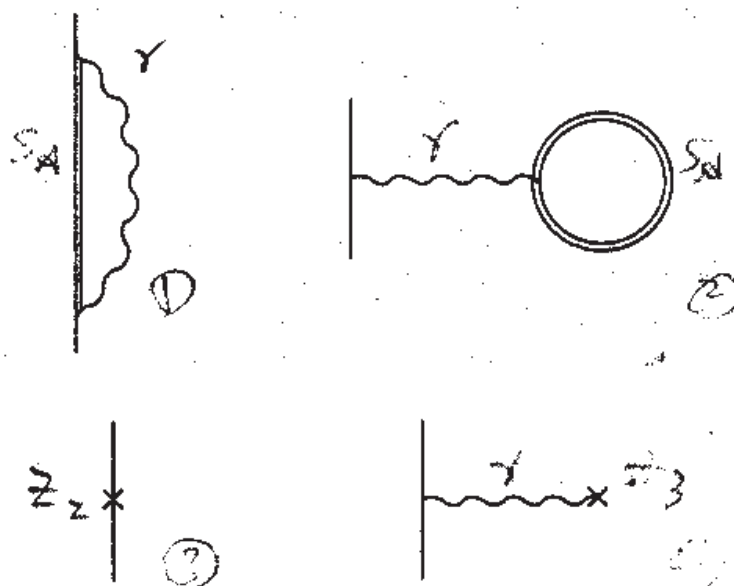
Figure 14.1. Lowest-order Feynman diagrams for the electron self-energy function \Sigma^*(x, y) in the presence of an external field. Here double straight lines represent electron propagators S_A that include effects of the external field; single straight lines are the incoming and outgoing electron lines; wavy lines are virtual photons; the cross represents renormalization counterterms.
