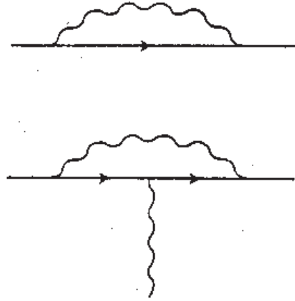
Figure 10.5. Diagrams for the first corrections to the electron propagator and vertex function in quantum electrodynamics. Here straight lines are electrons; wavy lines are photons.
