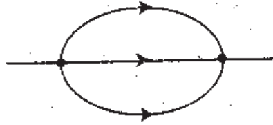
Figure 6.2. Example of a graph requiring extra combinatoric factors in the S -matrix. For an interaction involving, say, three factors of some field (as well as other fields) we usually include a factor 1/3! in the interaction Hamiltonian, to cancel factors arising from sums over ways of pairing these fields with their adjoints in other interactions. But in this diagram there are two such factors of 1/3! and only 3! different pairings, so we are left with an extra factor of 1/3! .
