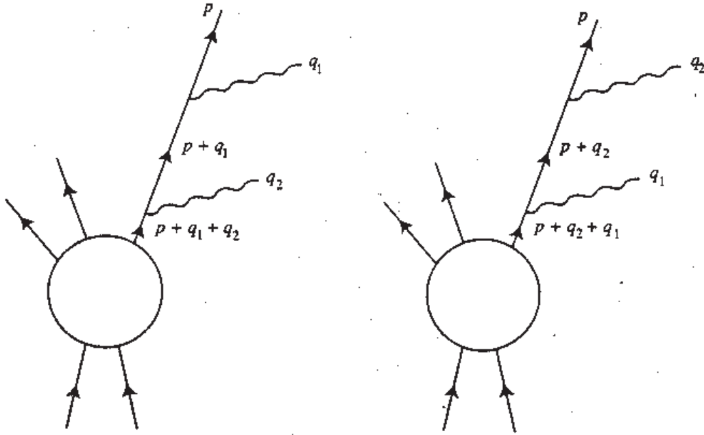
Figure 13.2. Graphs for the emission of two soft photons from the same outgoing charged particle. Straight lines are hard particles; wavy lines are soft photons.
