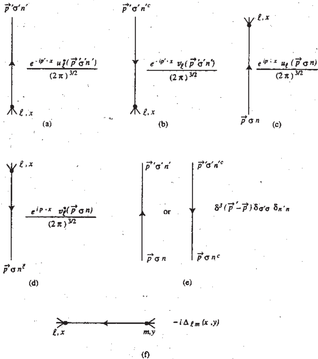
Figure 6.1. Graphical representation of pairings of operators arising in the coordinate-space evaluation of the S -matrix. The expressions on the right are the factors that must be included in the coordinate-space integrand of the S -matrix for each line of the Feynman diagram.
