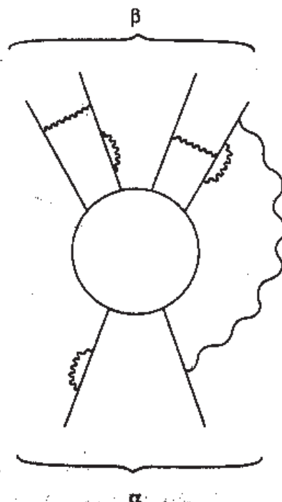
Figure 13.3. A typical dominant graph for the radiative corrections due to virtual soft photons to the S -matrix for the process \alpha \rightarrow \beta . Straight lines are particles in the states \alpha and \beta (including possible hard photons); wavy lines are soft photons.
